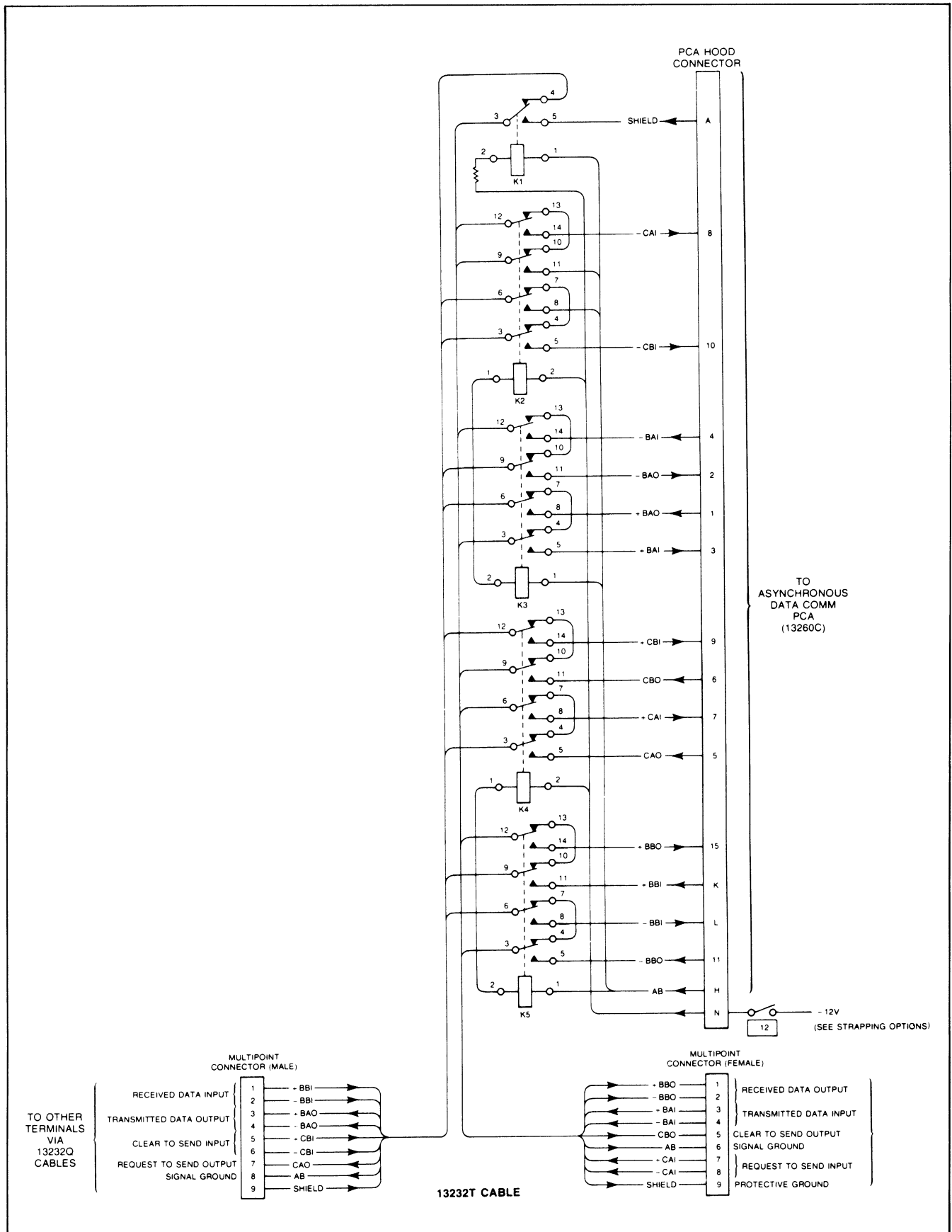
Figure 7-24. Power-Down-Protect Cabling for Asynchronous Multipoint Configuration
