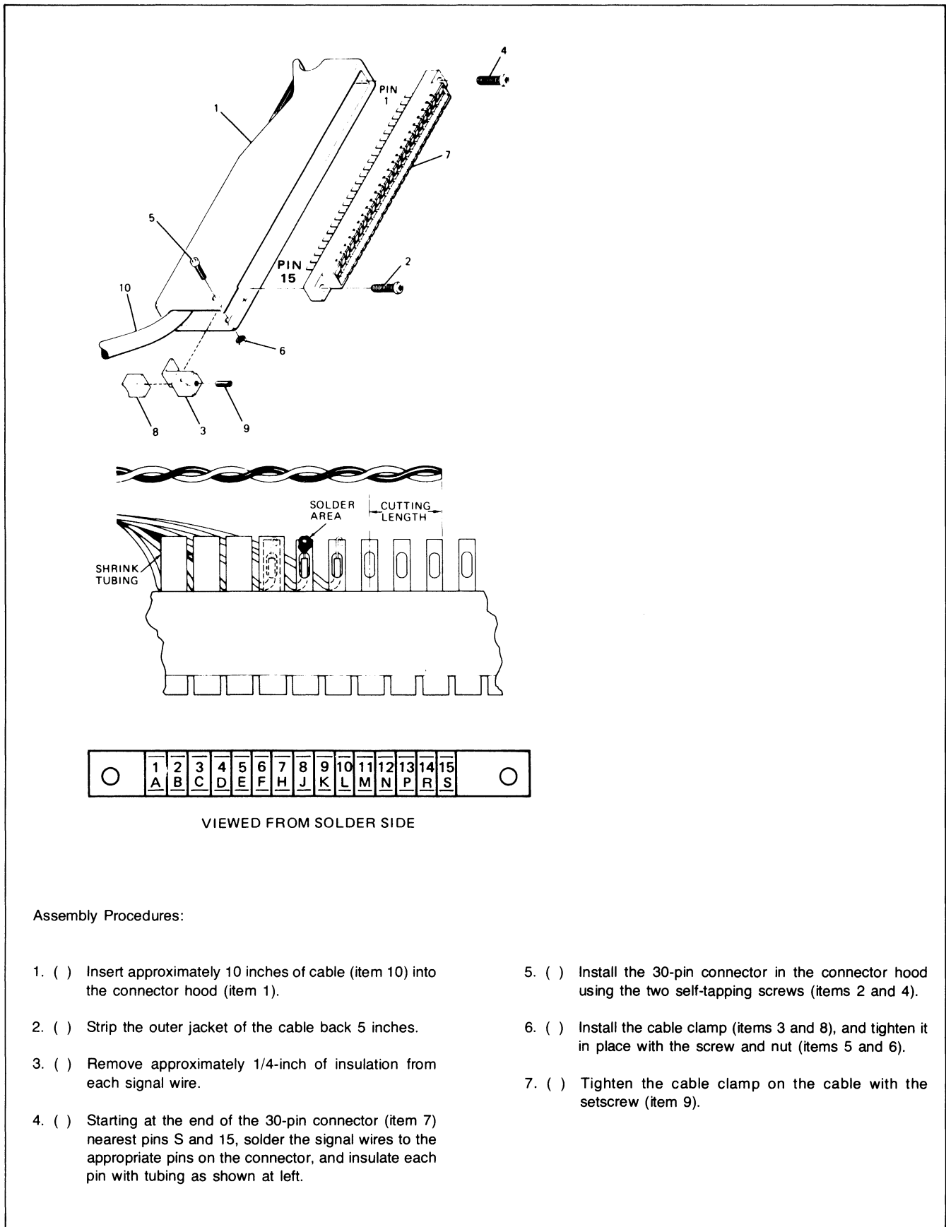
Figure 7-26. Assembling the PCA Hood Connector
