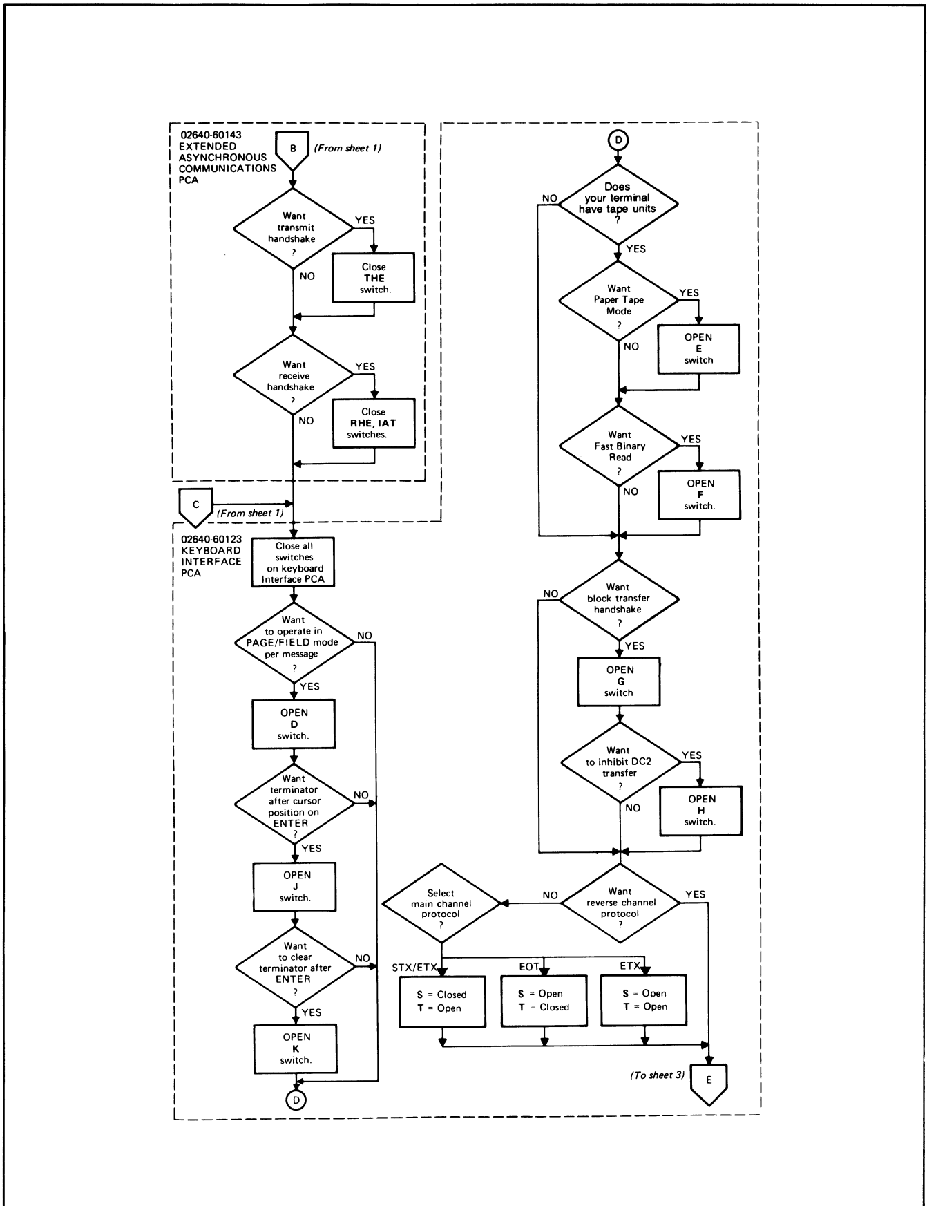
Figure 5-10. Point-to-Point Data Communications Configuration Flowchart (Sheet 2 of 4)
