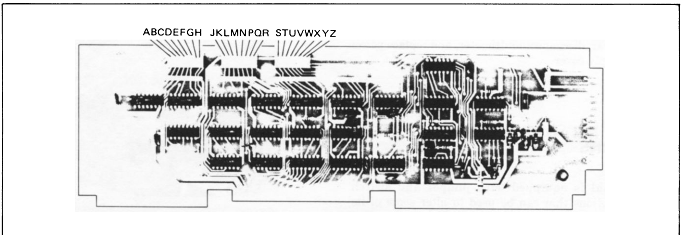
Figure 7-15. Keyboard Interface PCA Strapping Options
