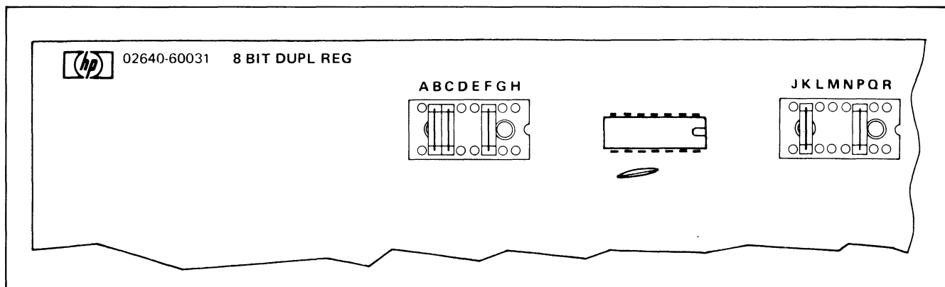
Figure 7-11. Terminal Duplex Register PCA Jumper Configuration
