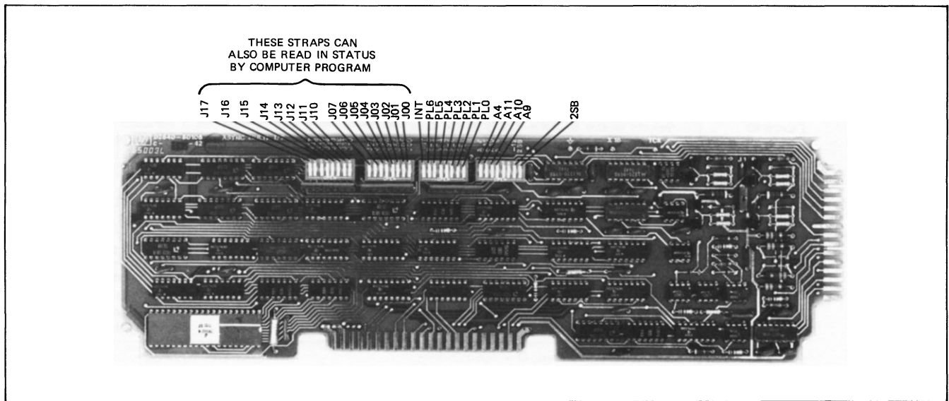
Figure 7-17. Asynchronous Multipoint Communications PCA Strapping Options
