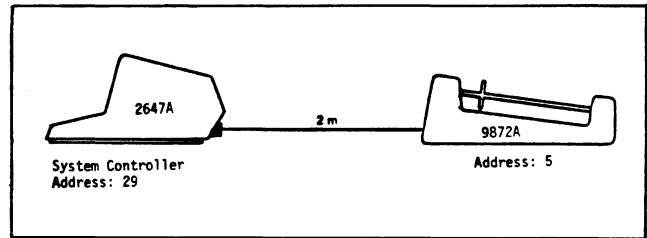
Figure 8-4. Terminal-to-Plotter Configuration
