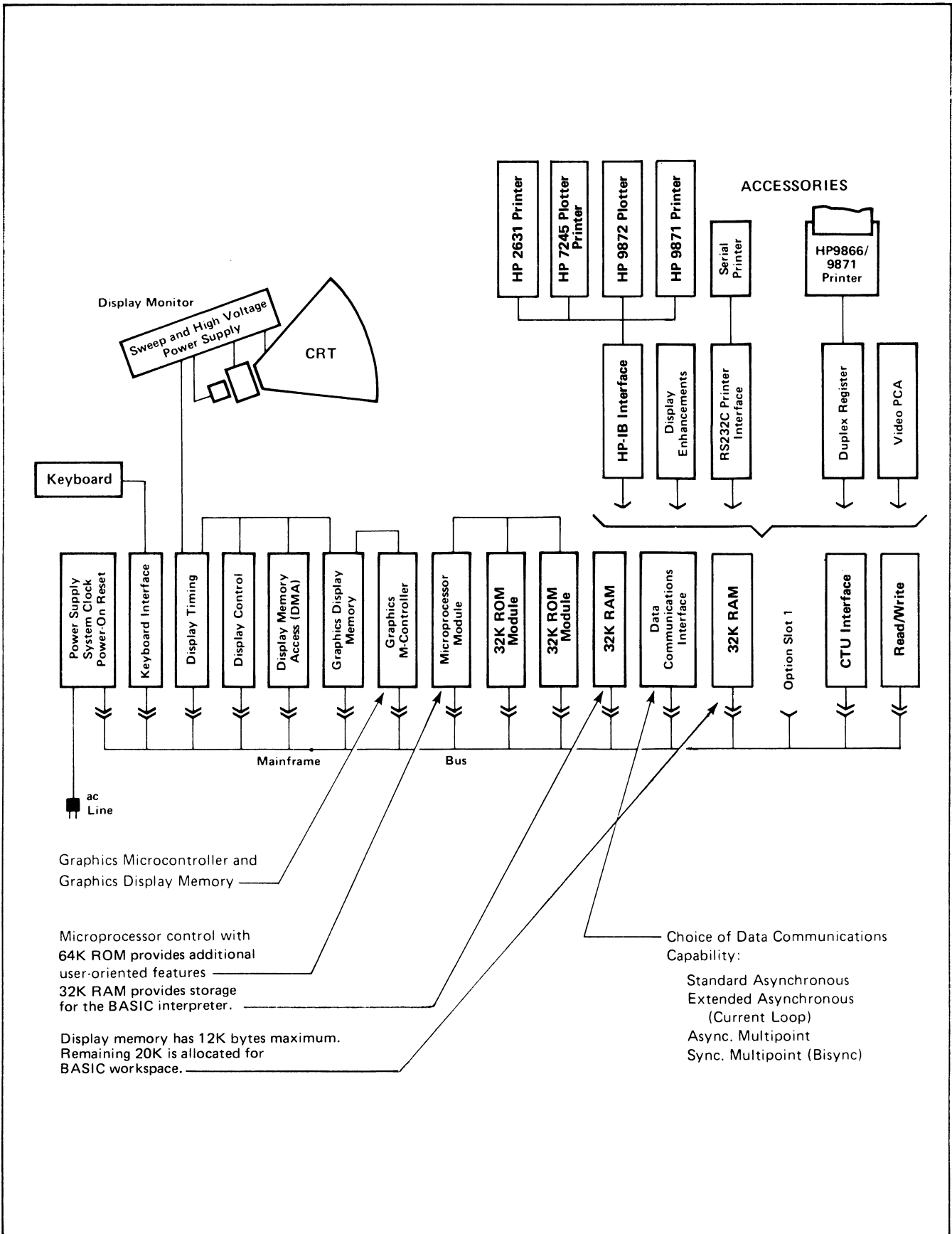
Figure 1-1. Terminal Architecture
