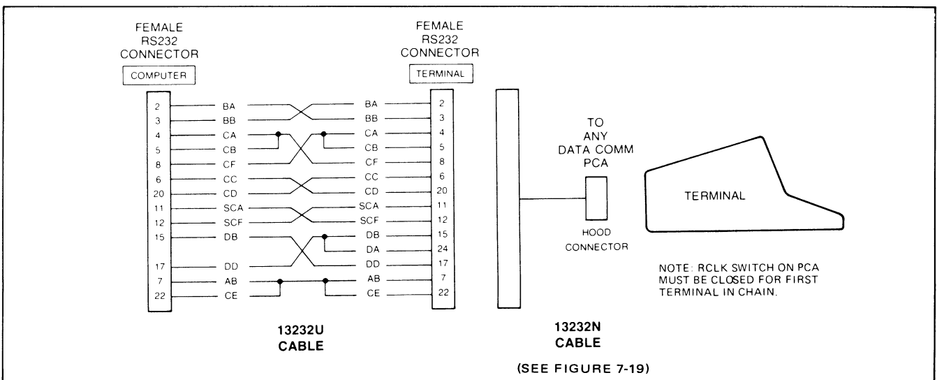
Figure 7-21. Modem By-Pass Cabling
