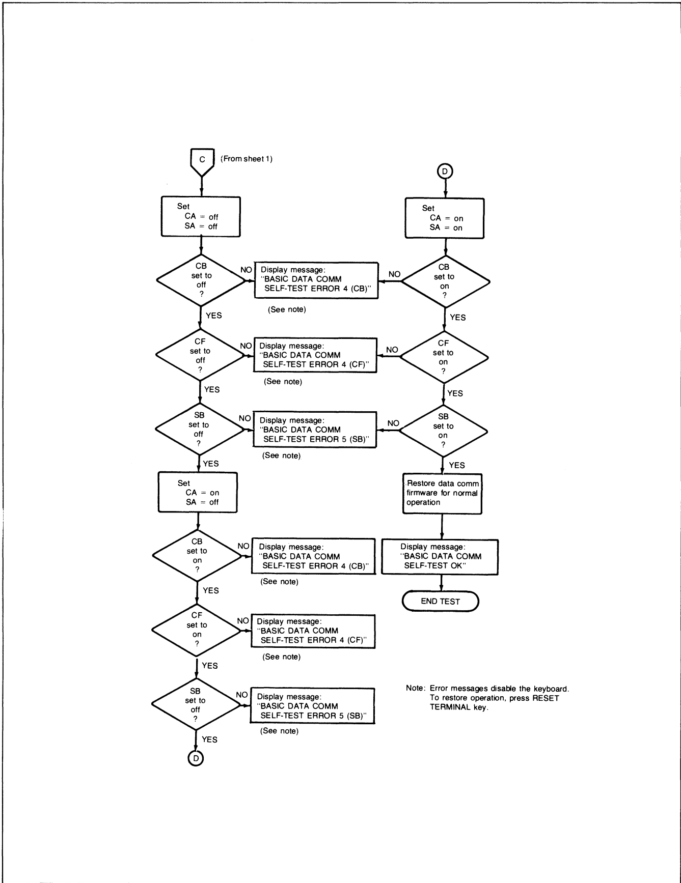
Figure 7-31. Basic Data Comm Self-Test Flowchart (Sheet 2 of 2)
